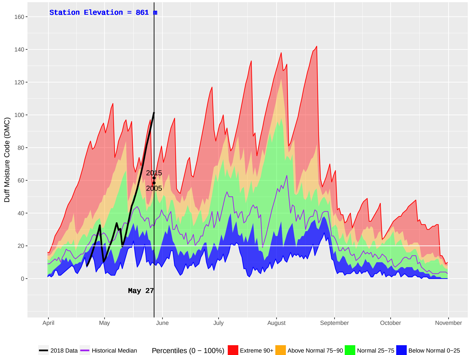
BLAEBERRY (866) : Historical (2004–2016) and Current (2018) Noon Duff Moisture Code (DMC)
